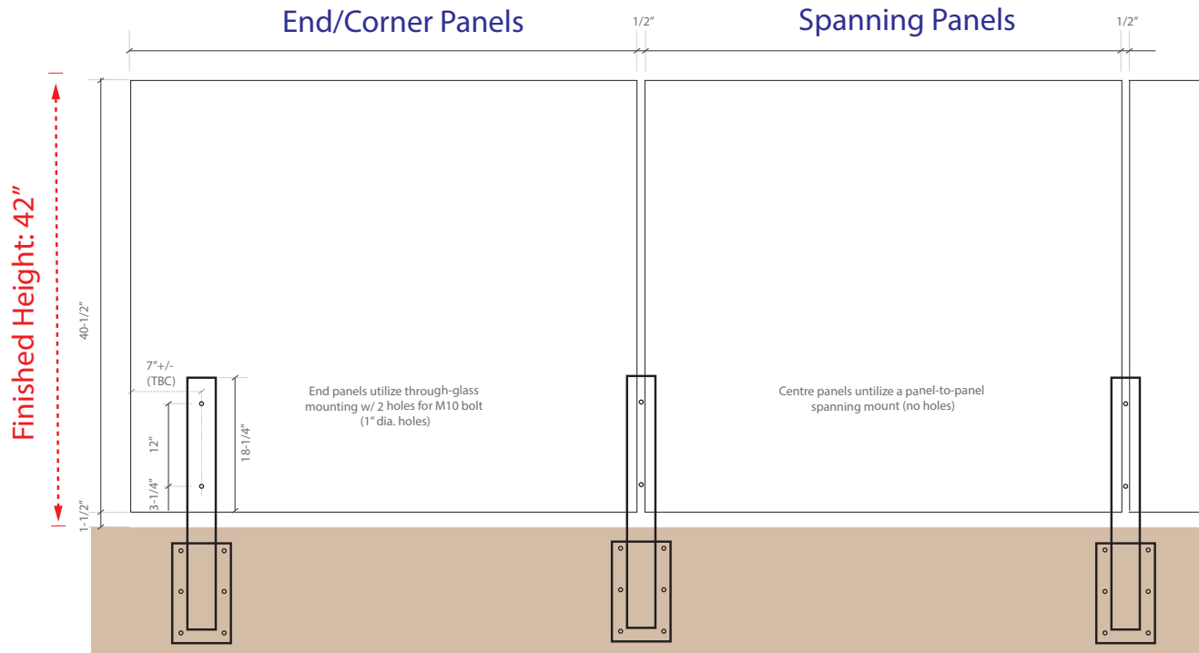
End/Corner Panels
